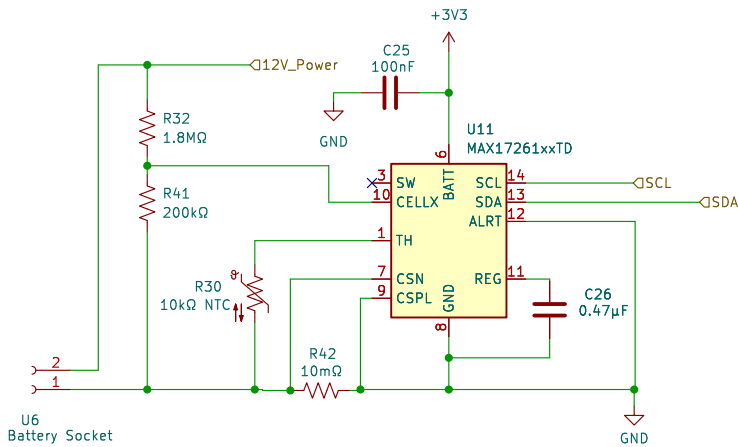
Battery Fuel Gauge
