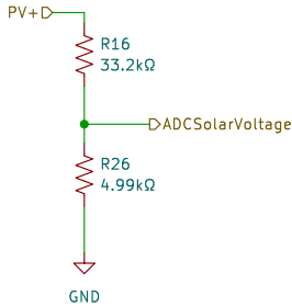
Measuring Solar panel Voltage
