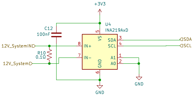
Measuring Voltage and Current After Power Switch
